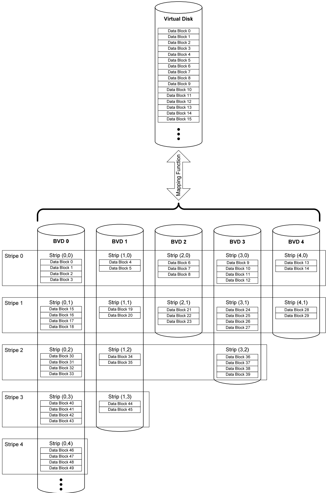
Figure 35: Spanned Secondary RAID Level (SRL=03)
