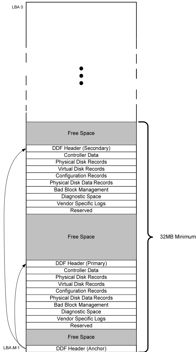
Figure 36: DDF Structure
